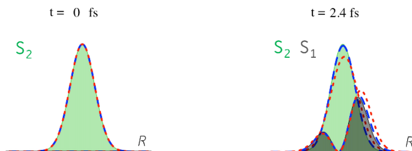
Рис. 1: The wavepacket population on the upper electronic state is plotted in light green, and in dark grey on the lower electronic state as a function of normal mode nuclear coordinate, R . The panels are computed for increasing time values as indicated. Shown also are two approximate computations where the surprisal is expanded in a minimal basis of dominant constraints \{\hat{\mathbb{I}}_N, \hat{a}, \hat{a}^\dagger, \hat{a}^\dagger \hat{a}\} , red dotted curve, and in an extended set \{\hat{\mathbb{I}}_N, \hat{a}, \hat{a}^\dagger, \hat{a}^2, (\hat{a}^\dagger)^2, \hat{a}^\dagger \hat{a}\} , blue dashed curve.
